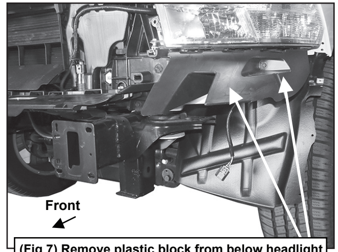
(Fig 7) Remove plastic block from below headlight
