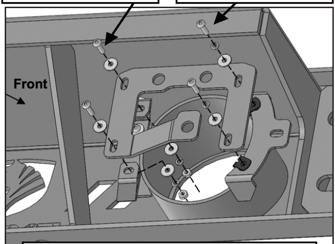
(Fig 14) Attach the factory fog light assembly to the Passenger/Right mounting location (3 post fog light mounting shown)
