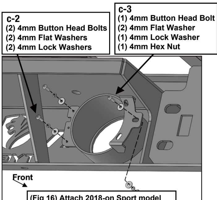
(Fig 16) Attach 2018-on Sport model fog light assembly to mounting plates, no adapters required. Passenger/Right Bumper illustrated
