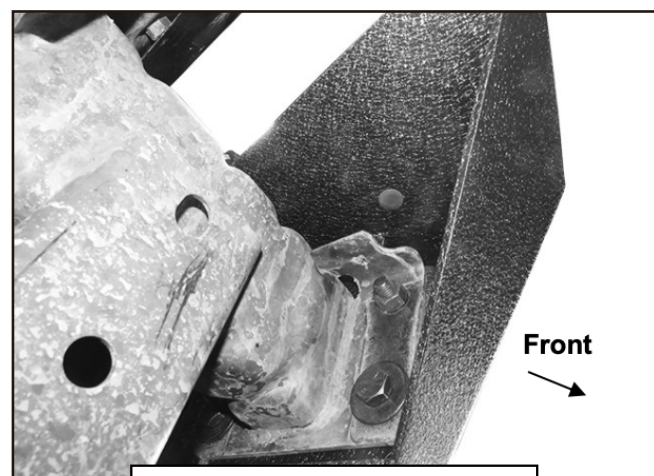
(Fig 21) Bumper attached to the Passenger/Right mounting plate
