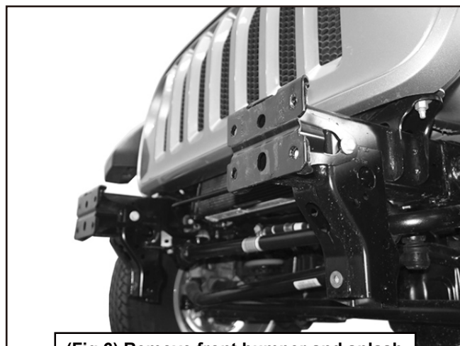
(Fig 6) Remove front bumper and splash guard or skid plate (2018-on JL pictured)
