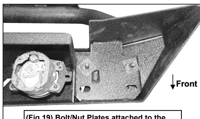
(Fig 19) Bolt/Nut Plates attached to the mounting plate on the back of the Bumper
