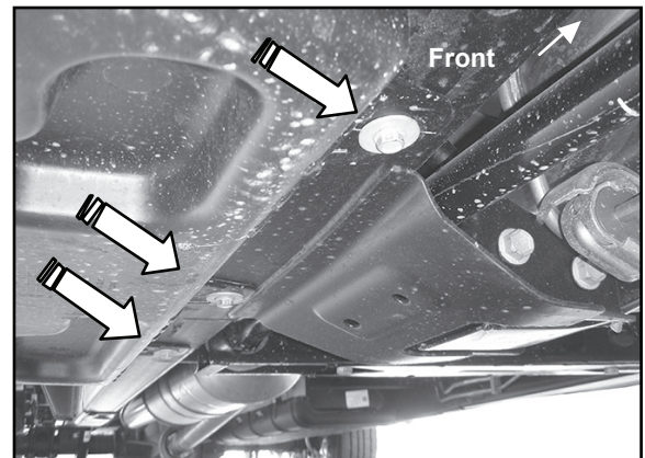
(Fig 10) 07-16 Passenger side front pictured with DEF tank cover. Remove (3) hex bolts to remove cover.
