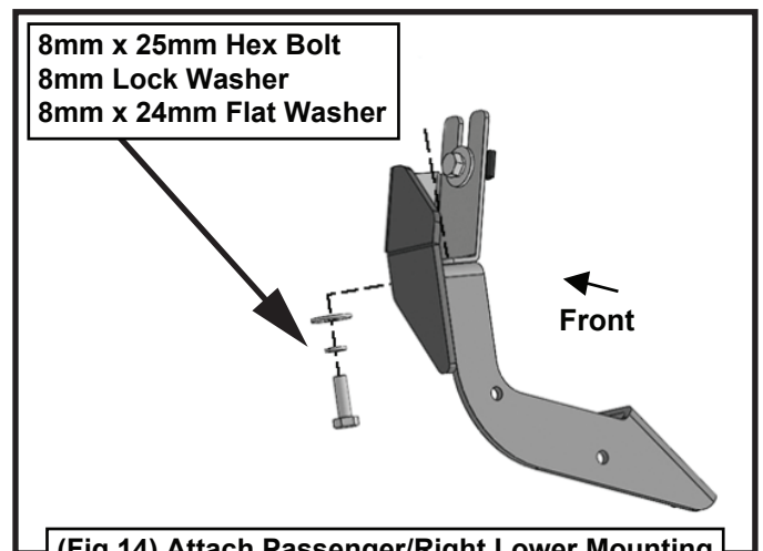
(Fig 14) Attach Passenger/Right Lower Mounting Bracket to the upper Mounting Bracket
