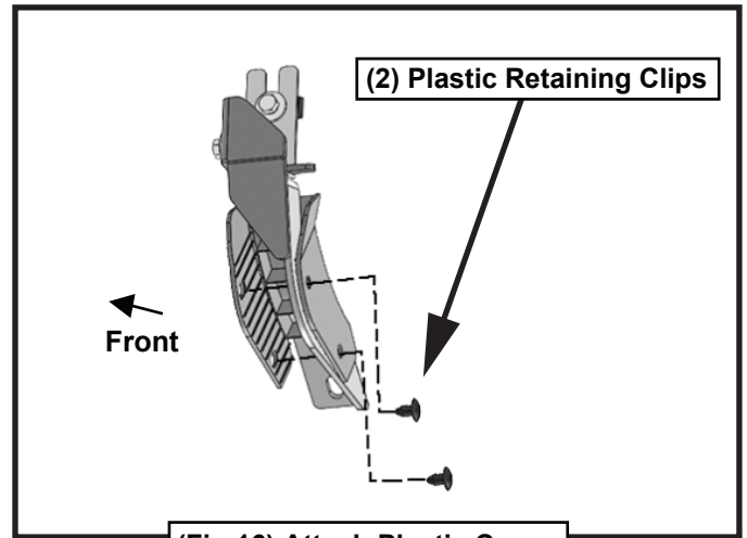
(Fig 16) Attach Plastic Cover to the Mounting Bracket
