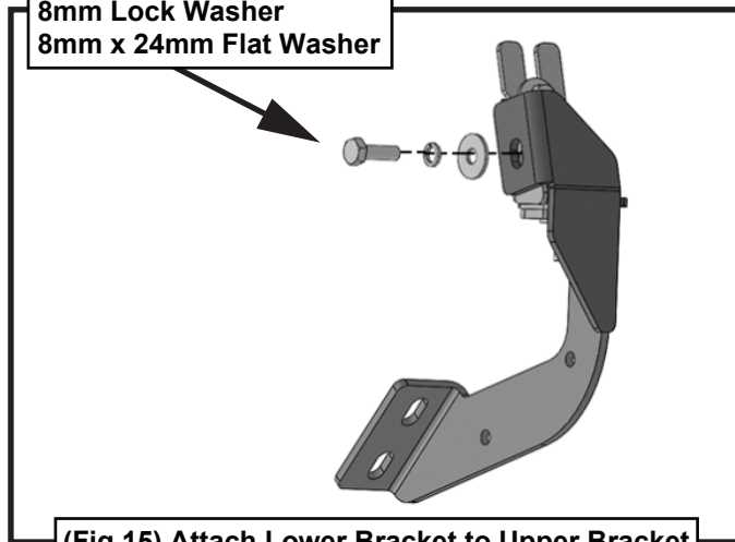
(Fig 15) Attach Lower Bracket to Upper Bracket
