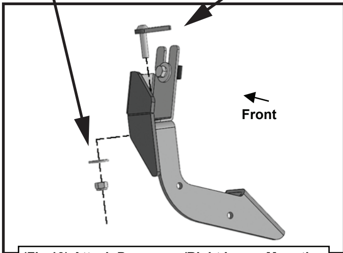
(Fig 13) Attach Passenger/Right Lower Mounting Bracket to the pinch weld and upper Mounting Bracket (models with hole in pinch weld shown)
