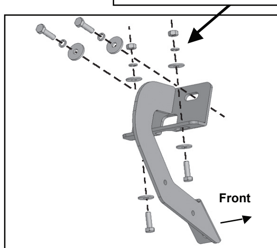
(Fig 3) Driver/left front mounting Bracket
