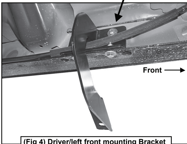
(Fig 4) Driver/left front mounting Bracket
