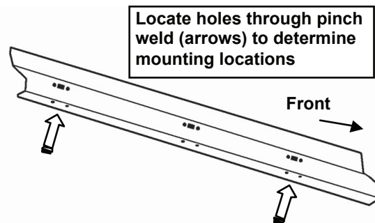
(Fig 1) Driver/left inner body panel illustrated
