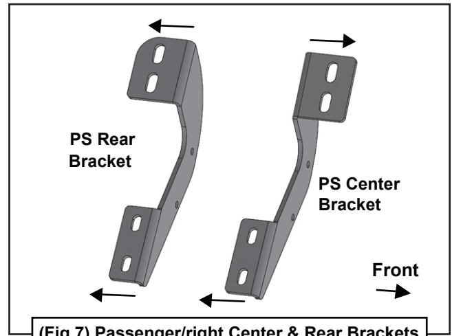
(Fig 7) Passenger/right Center & Rear Brackets
