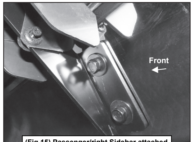
(Fig 15) Passenger/right Sidebar attached to PS Center Bracket
