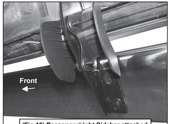
(Fig 16) Passenger/right Sidebar attached to PS Rear Bracket
