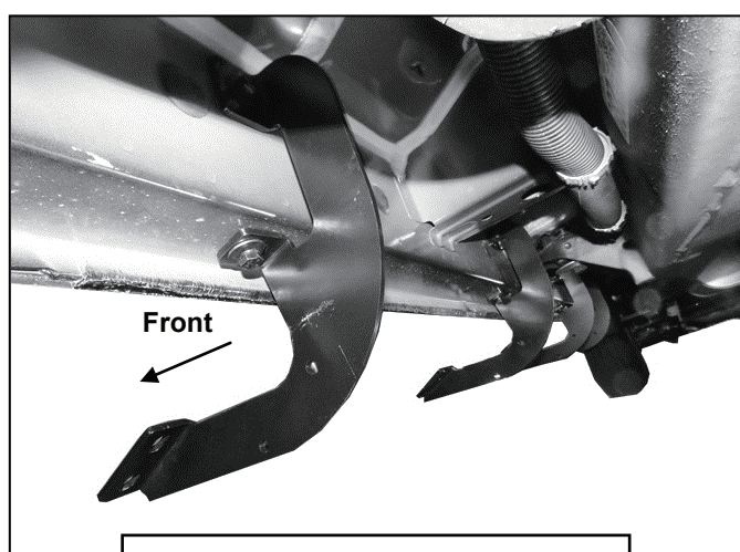
(Fig 7) Passenger Mounting Bracket
