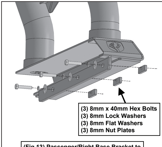
(Fig 13) Passenger/Right Base Bracket to bed installation
