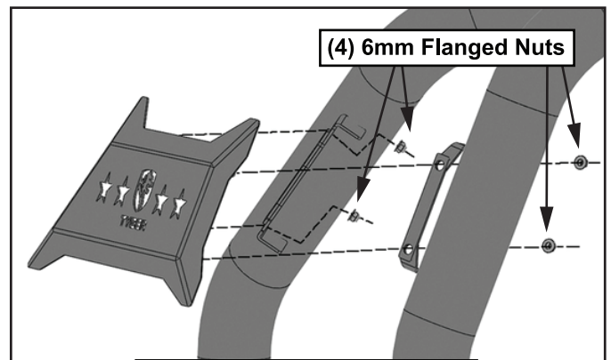
(Fig 7) Passenger/Right Decorative Plate installation
