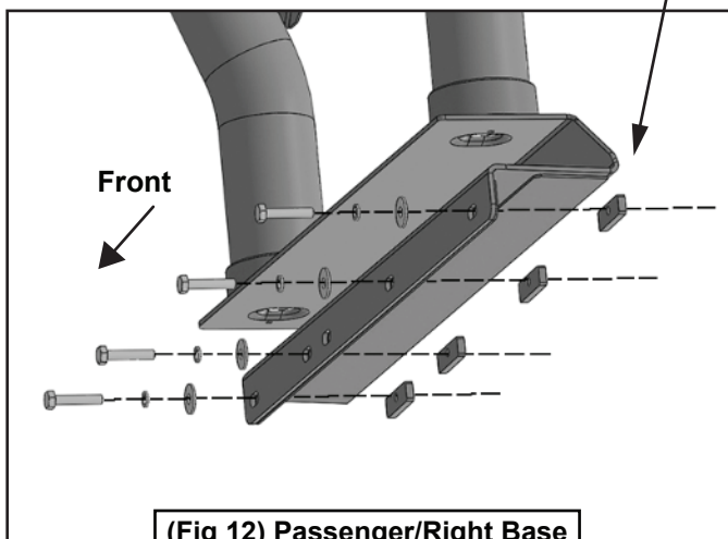
(Fig 12) Passenger/Right Base Bracket to bed installation
