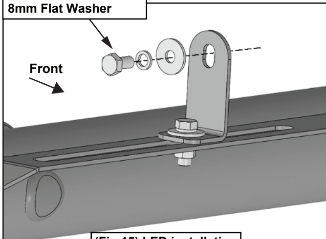
(Fig 15) LED installation
