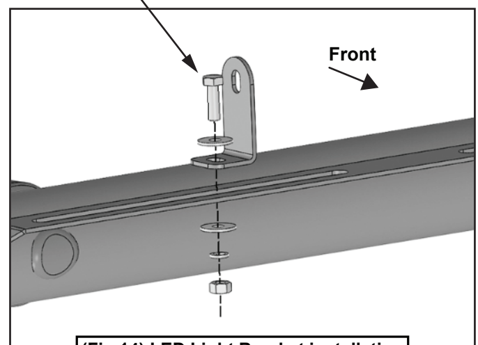
(Fig 14) LED Light Bracket installation
