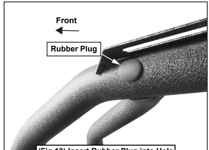
(Fig 13) Insert Rubber Plug into Hole
