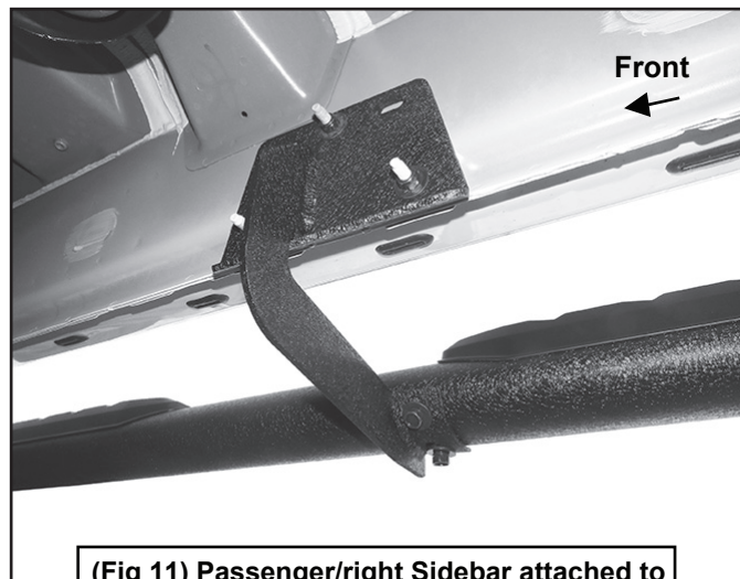
(Fig 11) Passenger/right Sidebar attached to center Bracket
