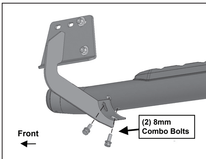
(Fig 9) Attach passenger/right Sidebar to front Bracket
