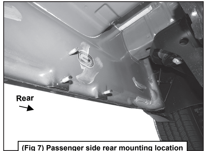
(Fig 7) Passenger side rear mounting location
