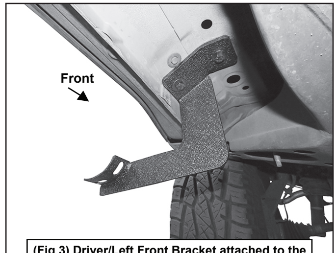
(Fig 3) Driver/Left Front Bracket attached to the floor panel
