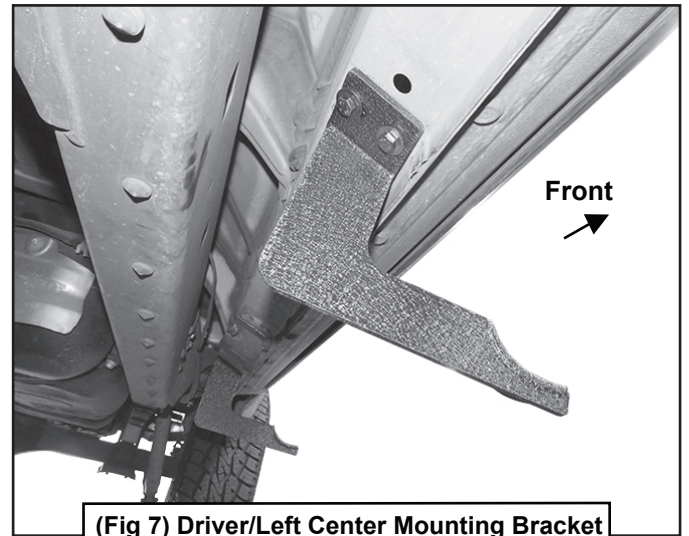
(Fig 7) Driver/Left Center Mounting Bracket attached to the floor panel
