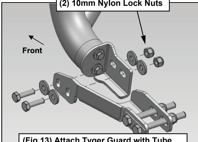
(Fig 13) Attach Tyger Guard with Tube Brackets to inside of Mounting Brackets
