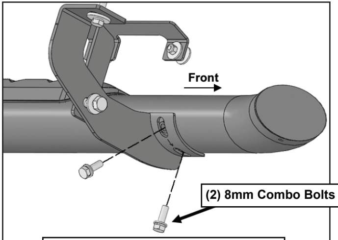
(Fig 15) Driver/Left Sidebar installation (Driver/Left front shown)
